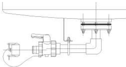
Outlet View
