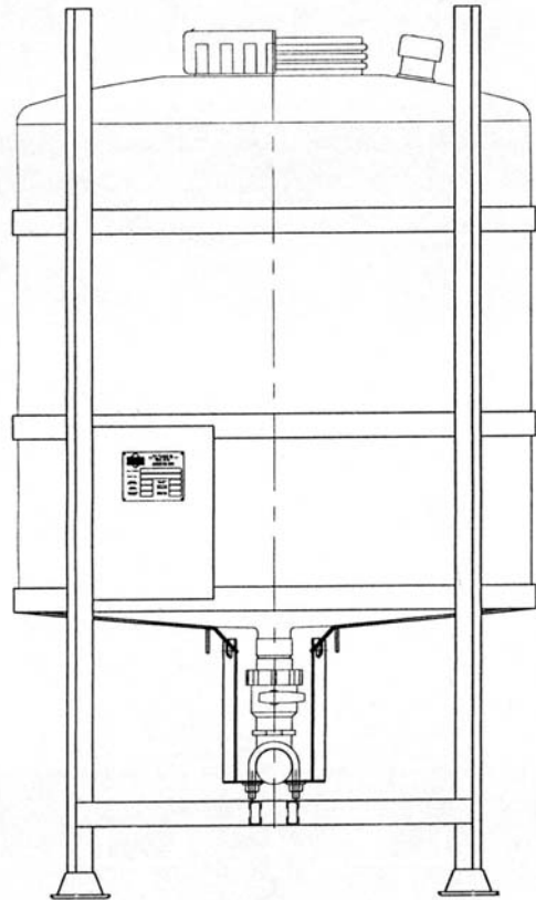
Front Elevation
