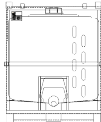
HGS 1000 Front elevation
